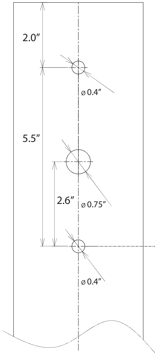
Mounting Pole Hole Dimensions
