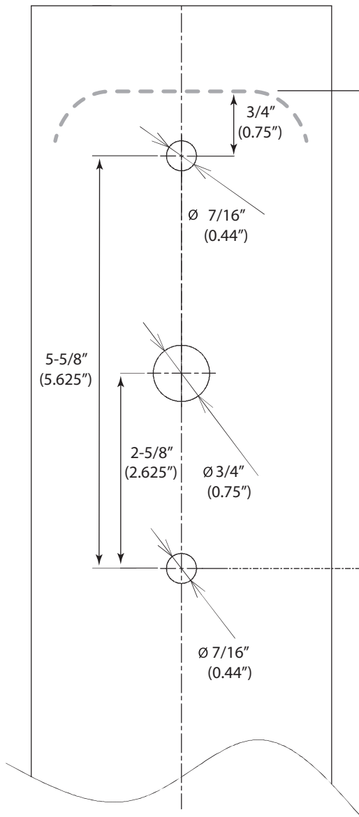
Mounting Pole Drilling Dimensions for New Construction
