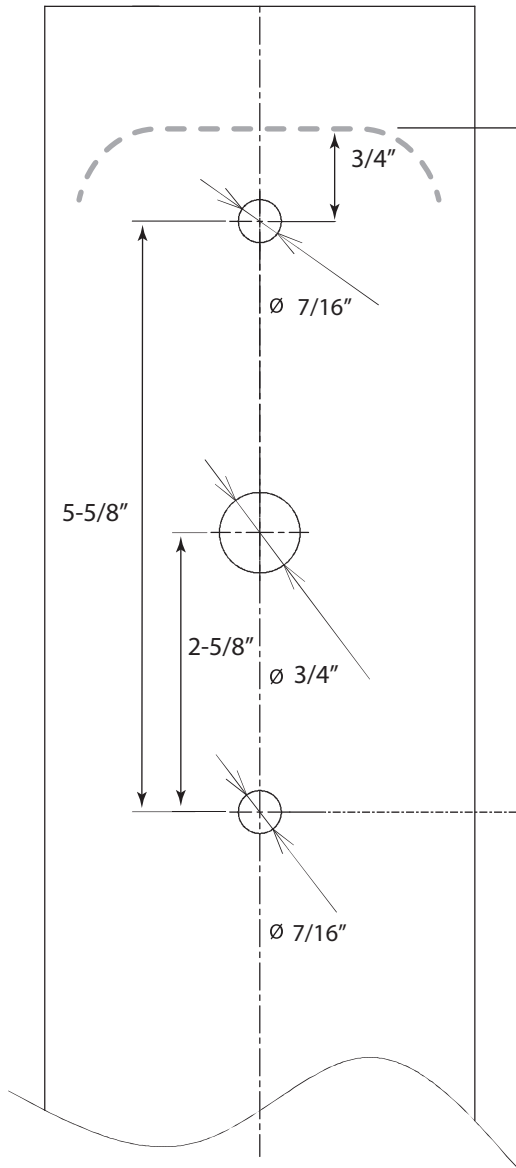
Mounting Pole Drilling Dimensions
